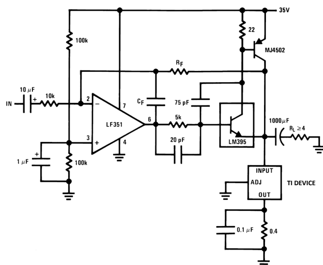
Figure 38. Tracking Preregulator
