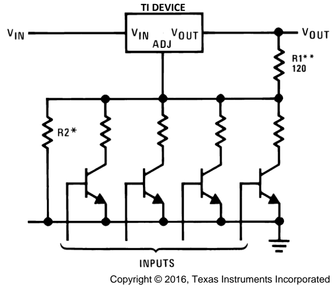
Figure 29. Digitally Selected Outputs
