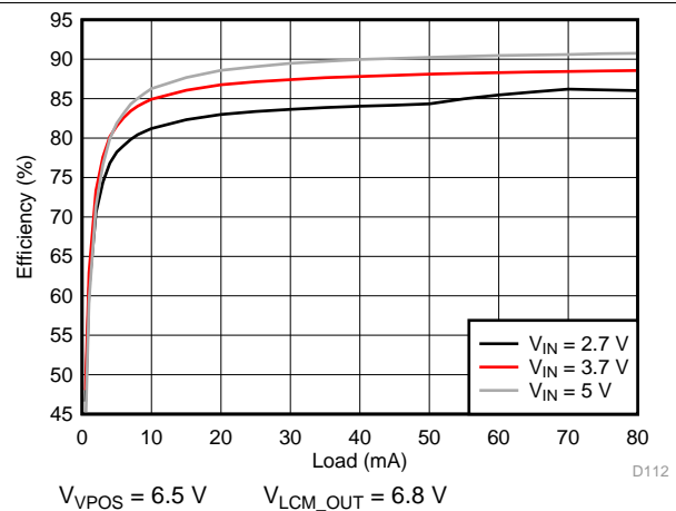
Figure 126. VPOS Efficiency
