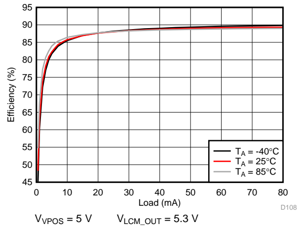
Figure 122. VPOS Efficiency
