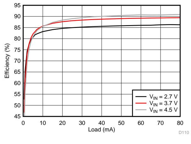
Figure 124. VPOS Efficiency
