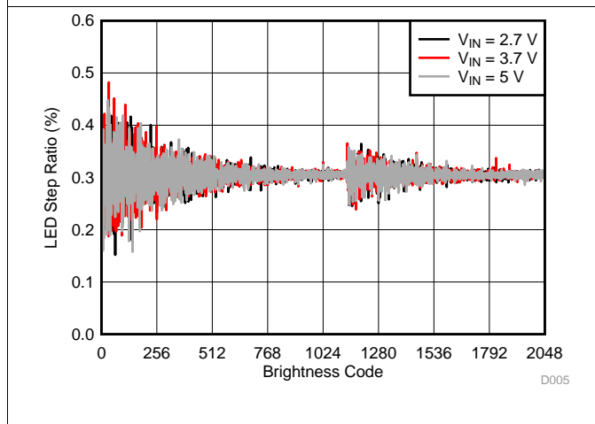
Figure 6. Backlight LED Current-Step Ratio
