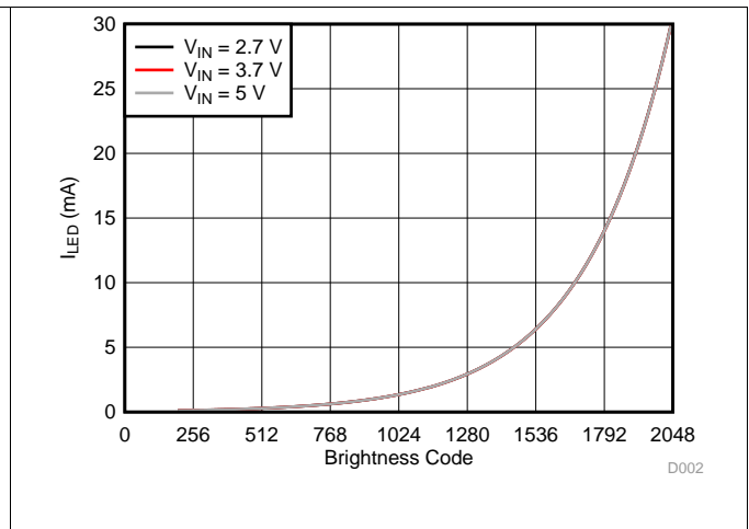
Figure 3. Backlight LED Current, Exponential Control
