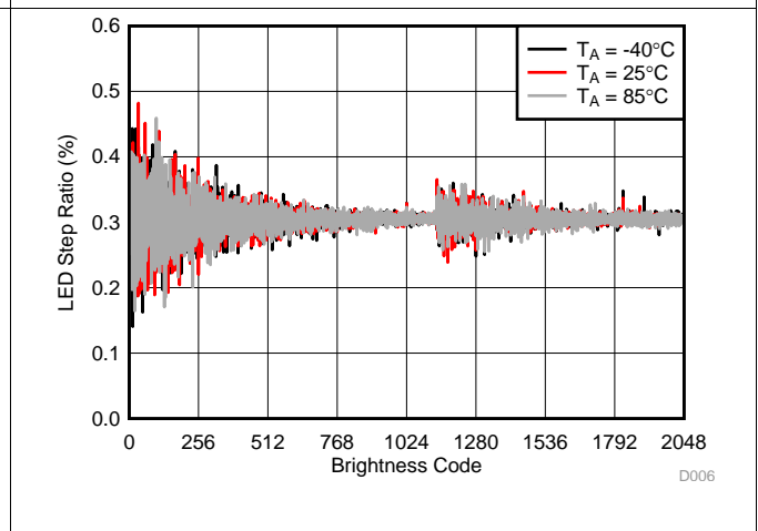
Figure 7. Backlight LED Current-Step Ratio
