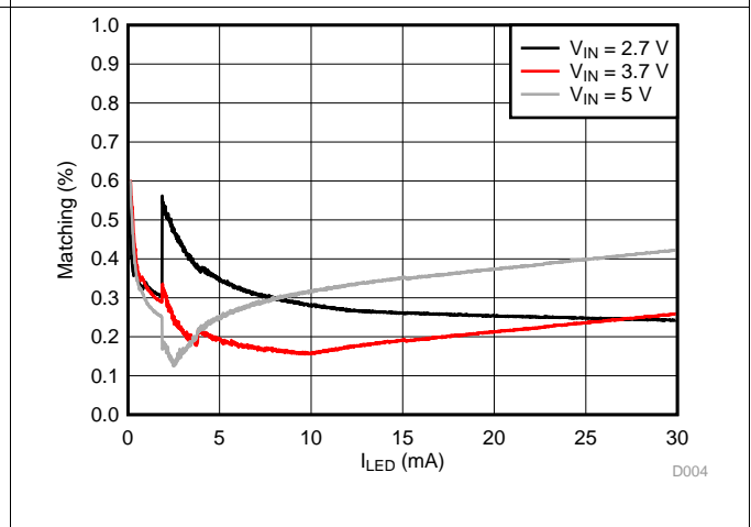
Figure 5. Backlight LED Current Matching
