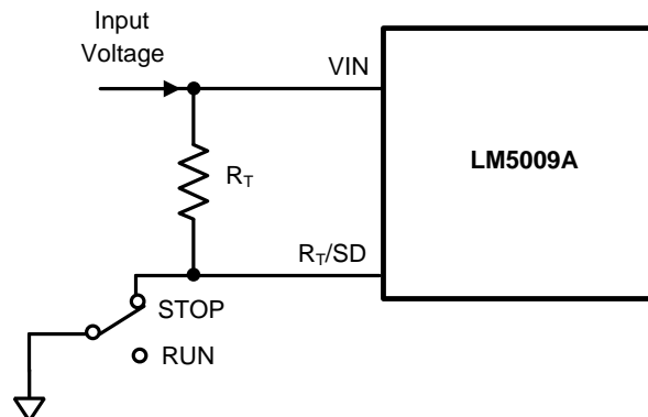
Figure 9. Shutdown Implementation
