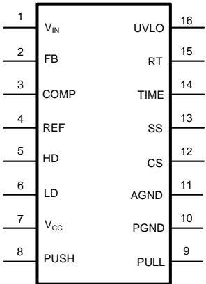
Figure 2. 16-Lead TSSOP or WSON See PW or NHQ0016A Package
