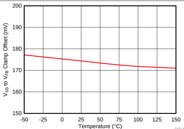
Figure 49. Soft-Start to Feedback Clamp Offset vs Temperature
