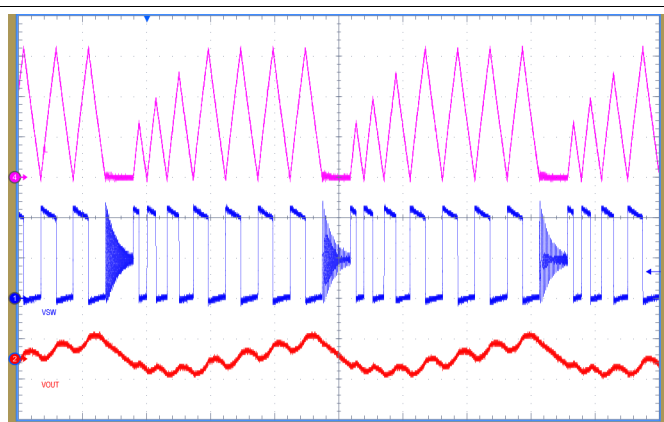
Figure 79. Converter Regulation
