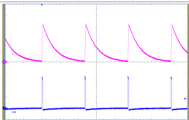
Figure 81. Full-Load Switching Waveforms
