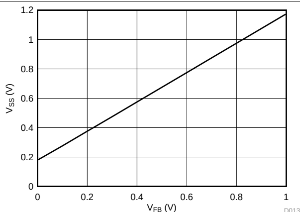
Figure 48. Soft-Start (SS) Voltage vs Feedback (FB) Voltage
