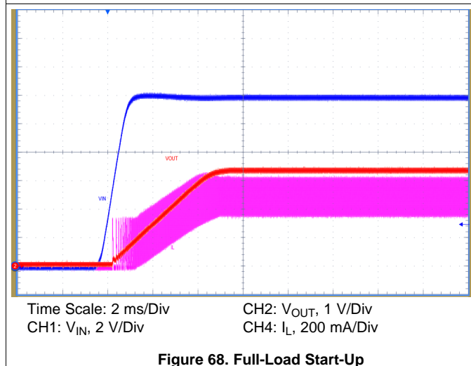
Figure 68. Full-Load Start-Up
