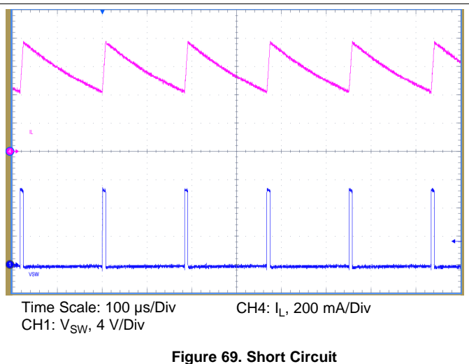
Figure 69. Short Circuit
