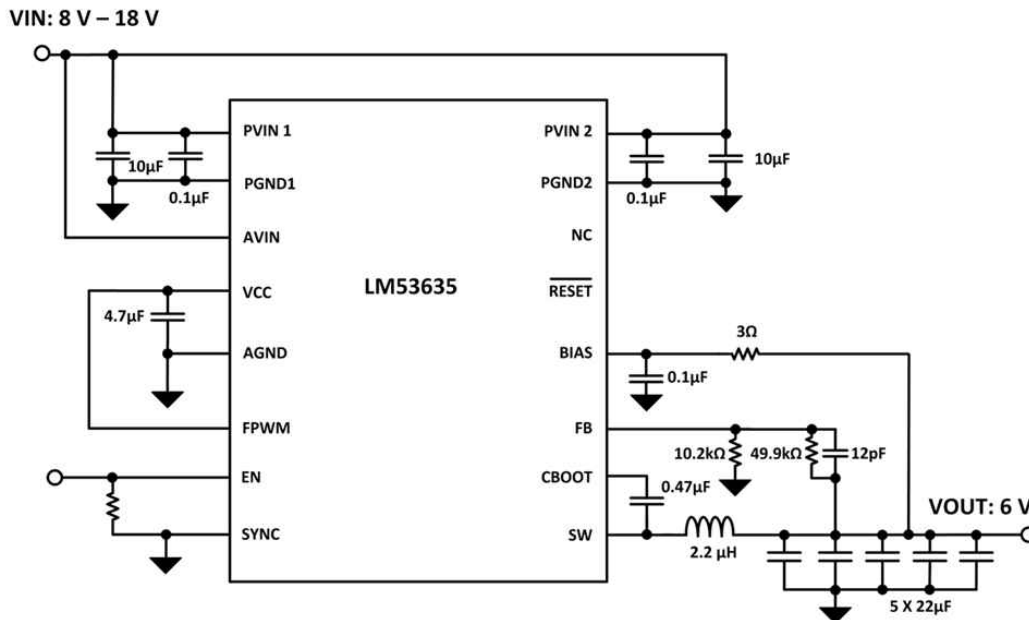
Figure 9-34. 6 V Output Power Supply
