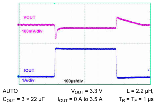
Figure 9-30. Load Transient
