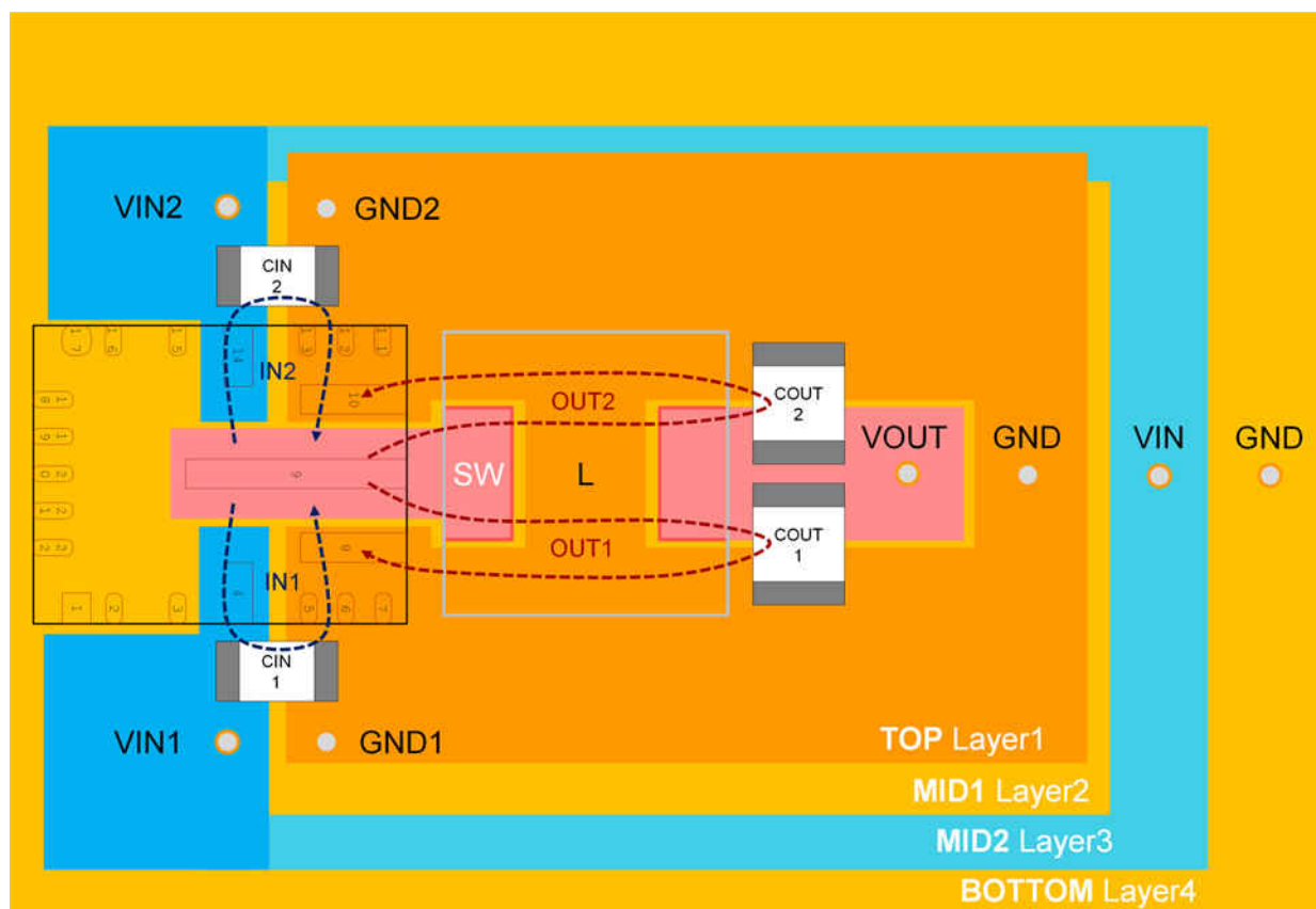
Figure 11-1. Layout of the Power Components and Current Flow
