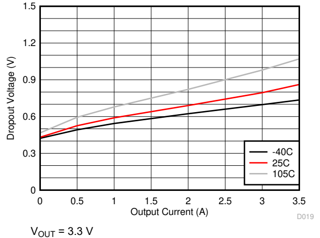
Figure 9-26. Dropout for \geq 1.85\text{ MHz}
