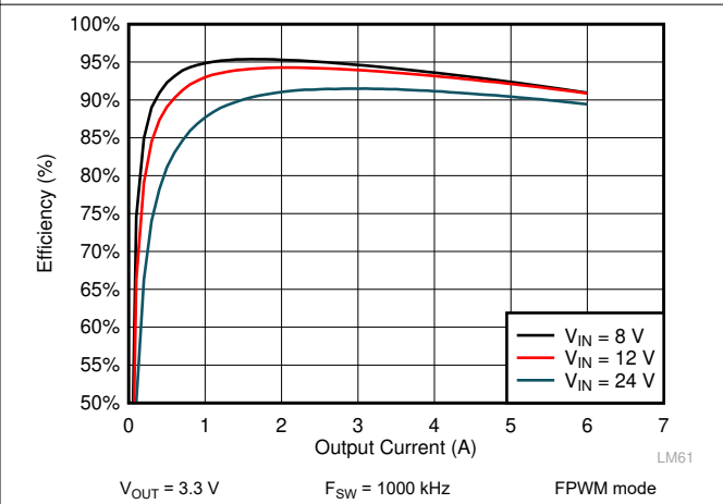
Figure 9-8. LM61460 Efficiency
