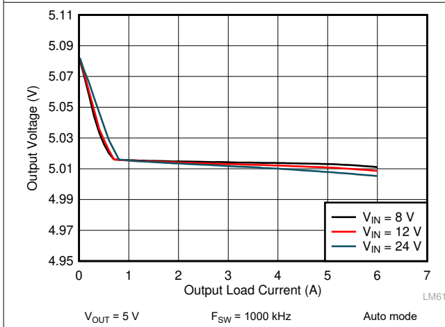
Figure 9-25. LM61460 Load and Line Regulation
