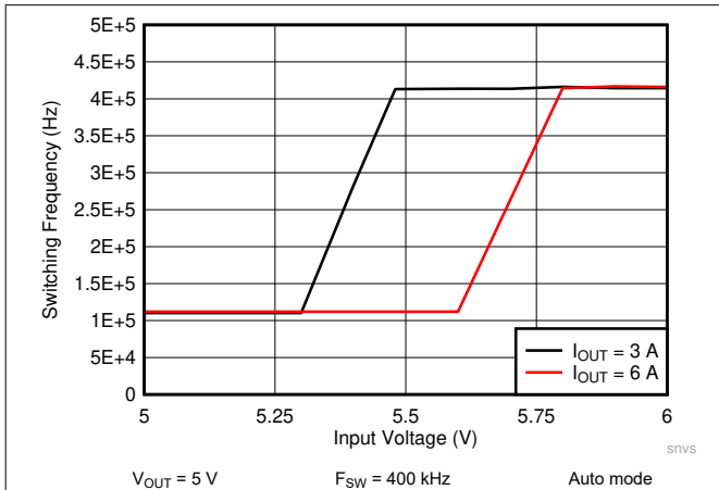
Figure 9-35. LM61460 Frequency Dropout Curve
