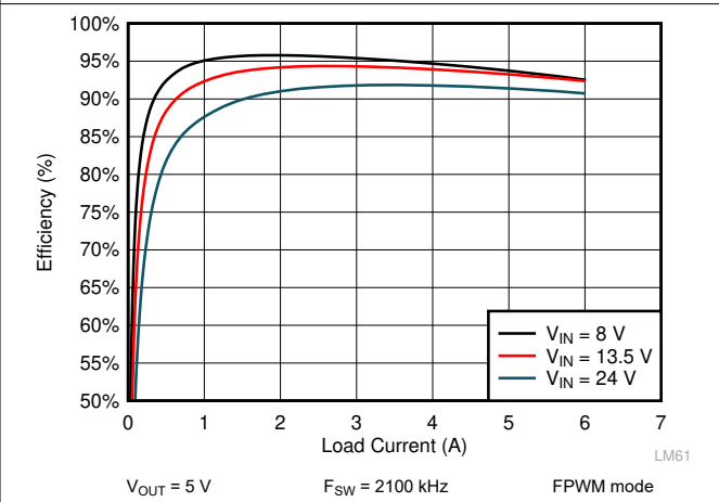
Figure 9-16. LM61460 Efficiency
