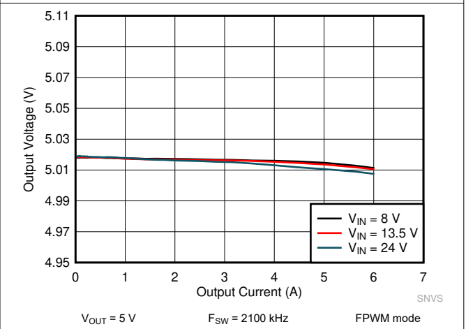
Figure 9-28. LM61460 Load and Line Regulation
