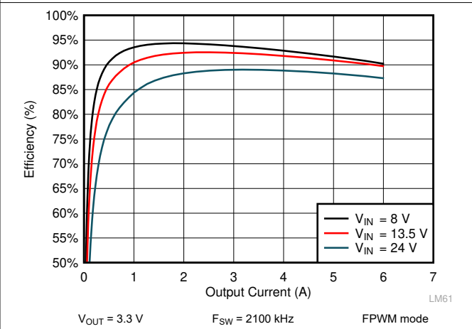
Figure 9-10. LM61460 Efficiency
