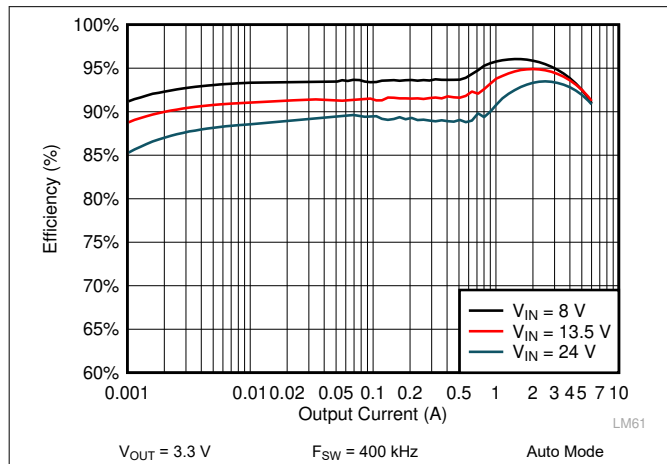
Figure 9-5. LM61460 Efficiency
