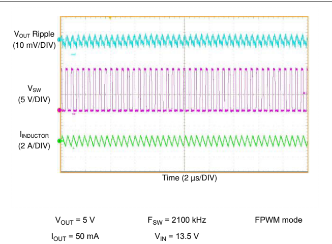
Figure 9-38. LM61460 Switching Waveform and V_{OUT} Ripple
