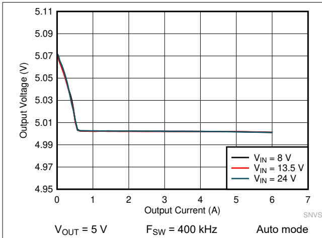
Figure 9-23. LM61460 Load and Line Regulation
