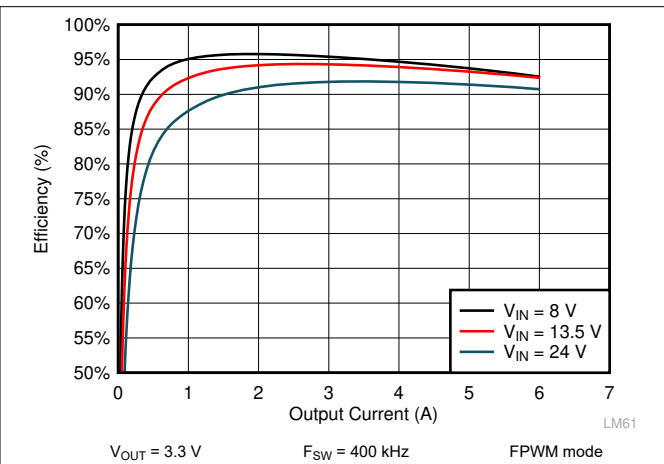
Figure 9-6. LM61460 Efficiency
