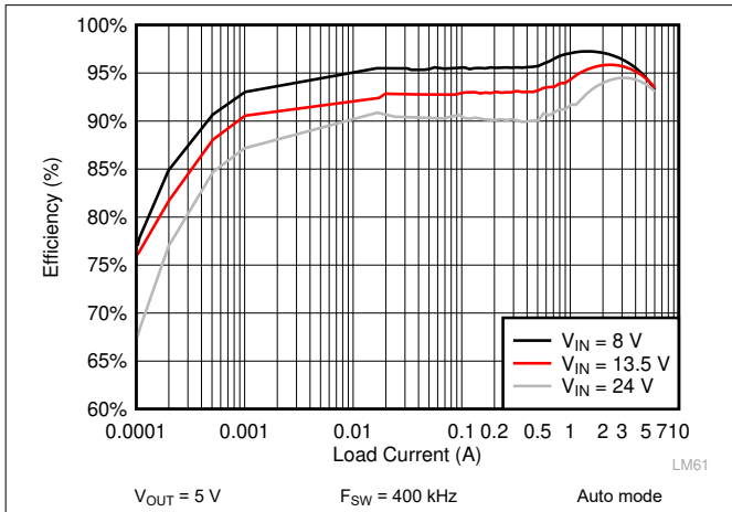
Figure 9-11. LM61460 Efficiency
