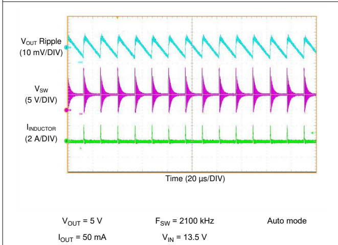
Figure 9-37. LM61460 Switching Waveform and V_{OUT} Ripple
