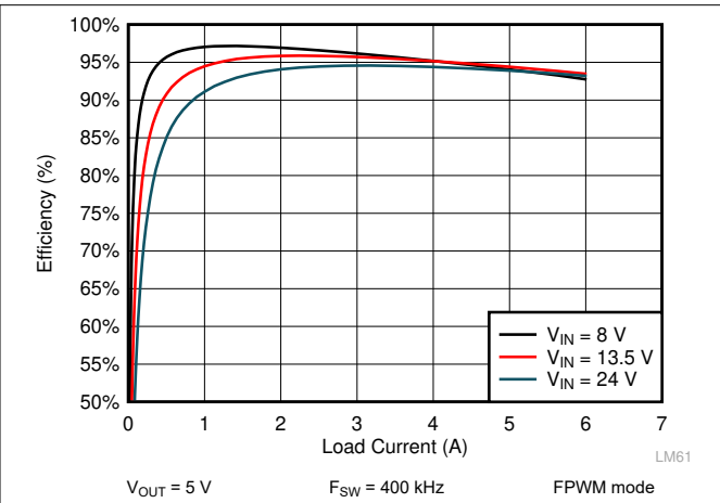
Figure 9-12. LM61460 Efficiency
