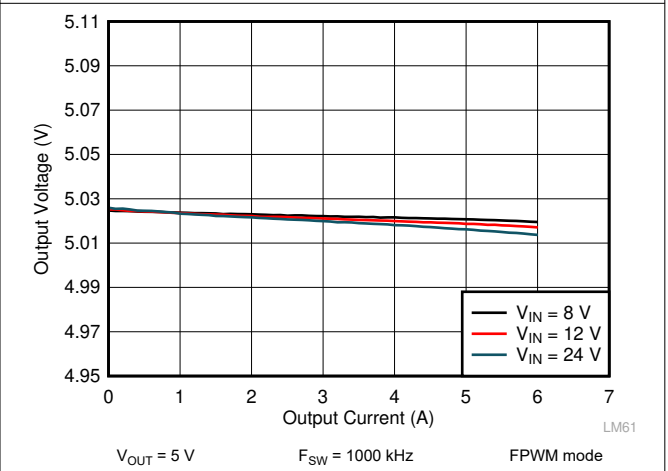
Figure 9-26. LM61460 Load and Line Regulation
