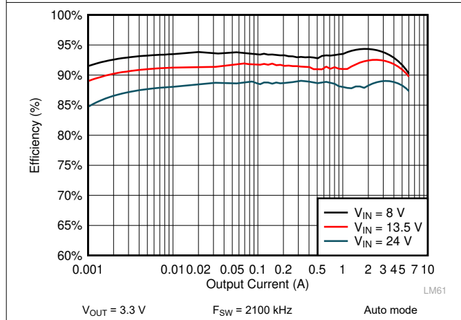
Figure 9-9. LM61460 Efficiency
