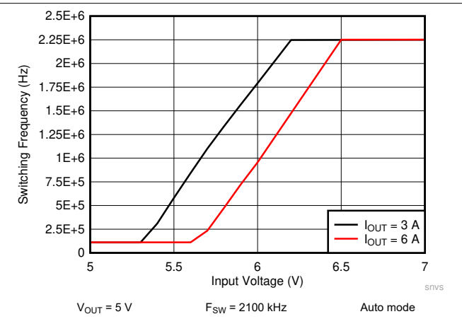
Figure 9-36. LM61460 Frequency Dropout Curve
