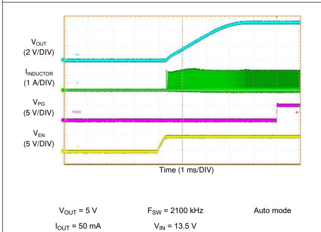
Figure 9-39. LM61460 Start-up with 50-mA Load
