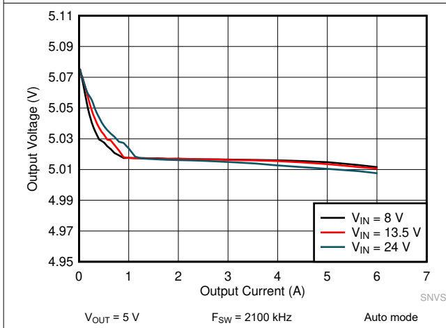
Figure 9-27. LM61460 Load and Line Regulation
