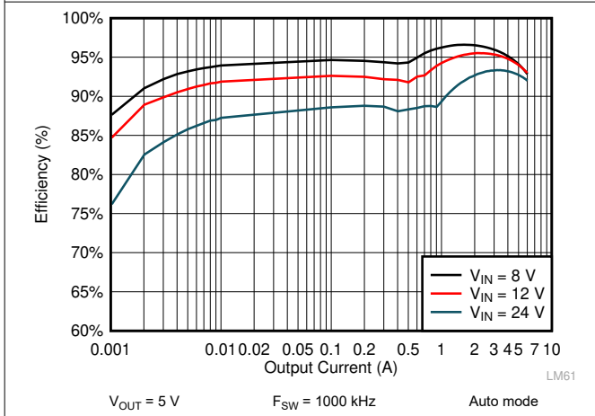
Figure 9-13. LM61460 Efficiency
