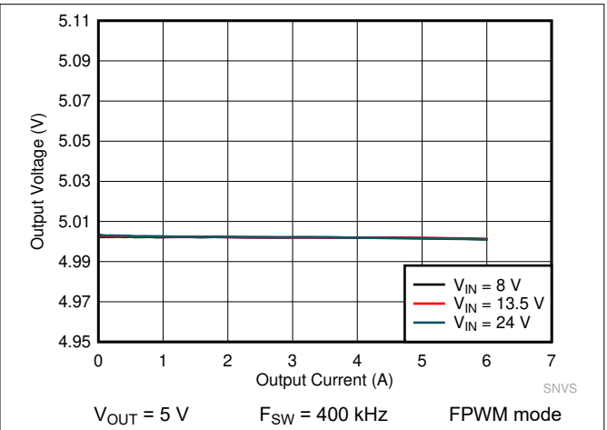
Figure 9-24. LM61460 Load and Line Regulation
