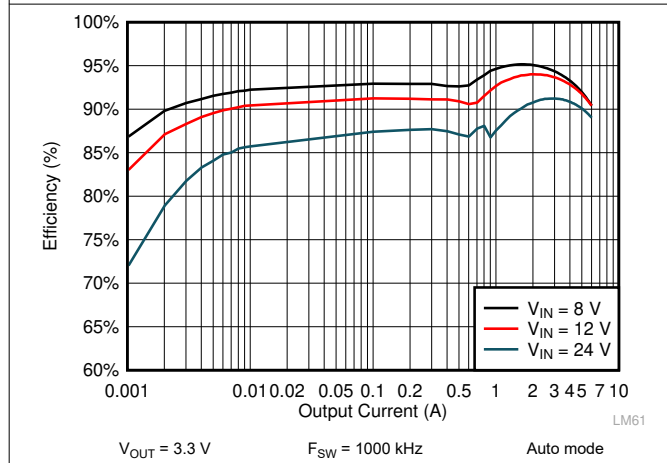
Figure 9-7. LM61460 Efficiency
