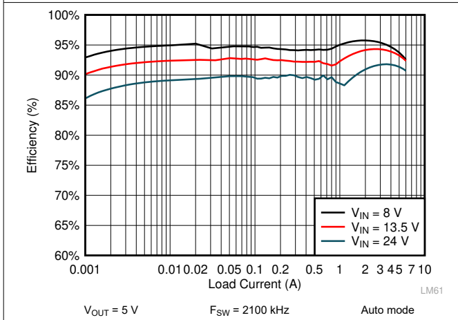
Figure 9-15. LM61460 Efficiency
