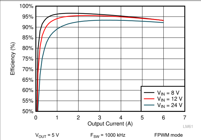
Figure 9-14. LM61460 Efficiency
