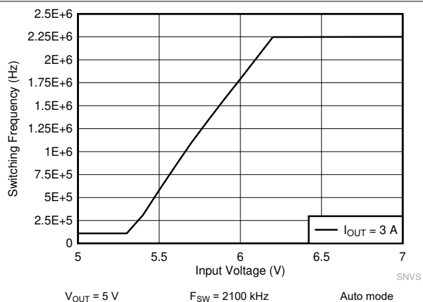
Figure 10-16. LM62440-Q1 Frequency Dropout Curve
