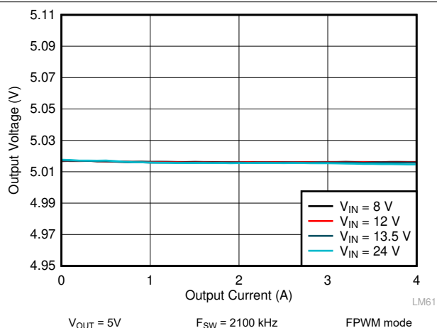
Figure 10-12. LM62440-Q1 Load and Line Regulation
