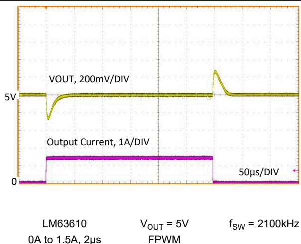
Figure 8-15. Load Transient
