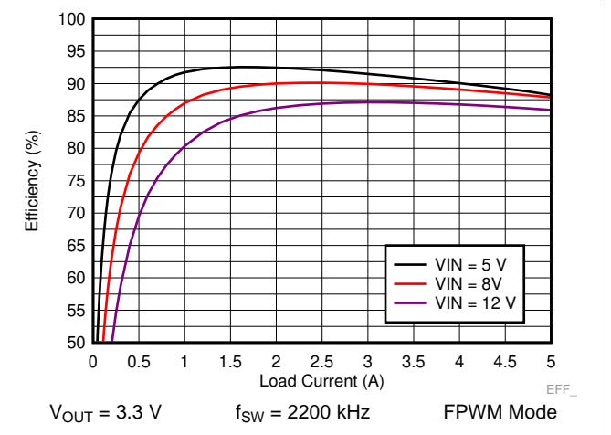
Figure 30. LM73605 Efficiency
