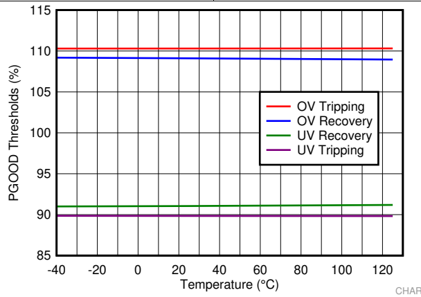
Figure 9. PGOOD Thresholds
