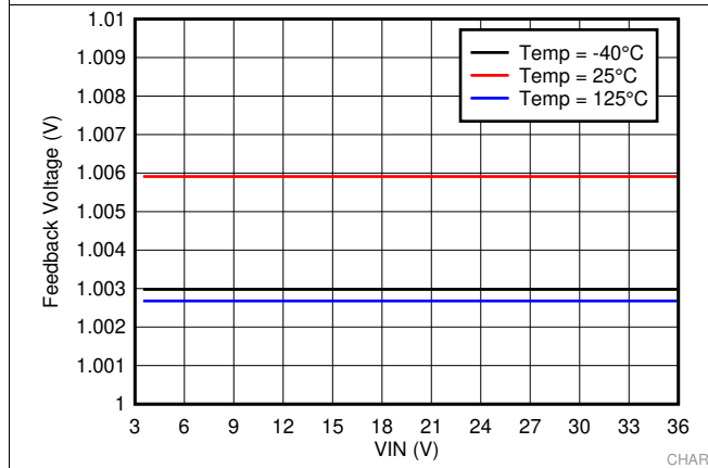
Figure 3. Feedback Voltage
