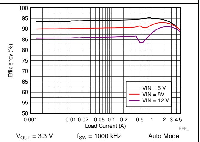
Figure 32. LM73605 Efficiency
