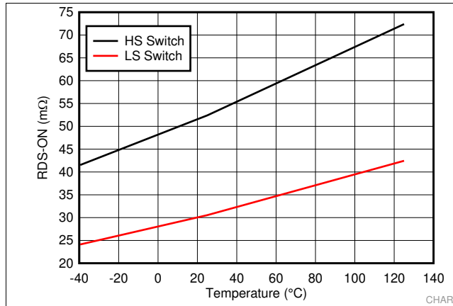
Figure 1. High-Side and Low-Side Switches R_{DS-ON}
