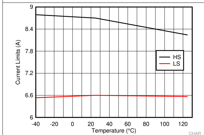
Figure 5. LM73605 High-Side and Low-Side Current Limit
