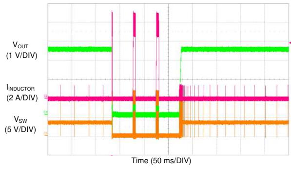
Figure 64. LM73606 Short-Circuit Hiccup Protection and Recovery
