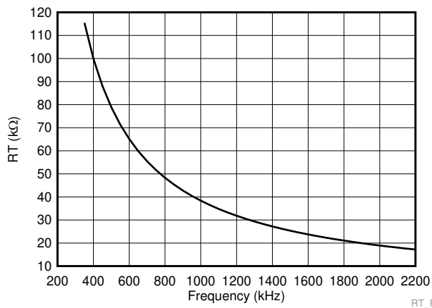
Figure 21. R_T Resistance versus Switching Frequency
