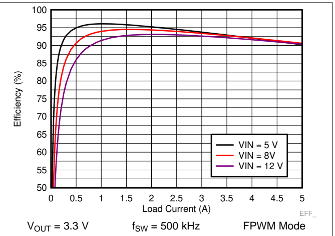
Figure 28. LM73605 Efficiency
