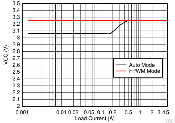
Figure 17. VCC Voltage versus Load Current
