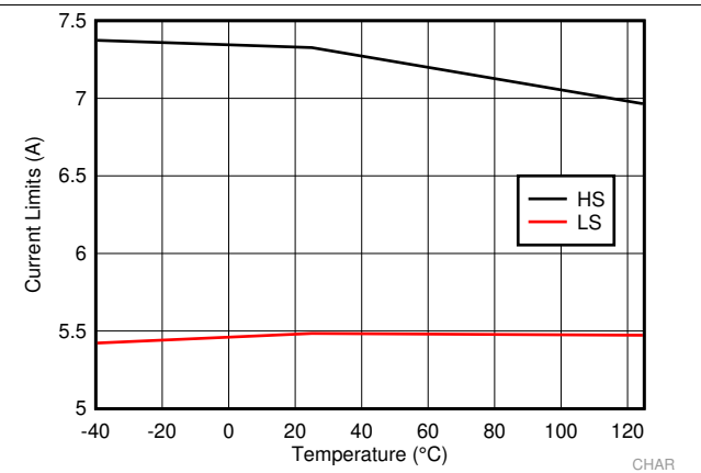
Figure 4. LM73605 High-Side and Low-Side Current Limits
