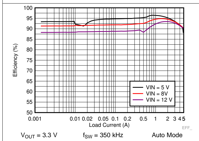
Figure 31. LM73605 Efficiency
