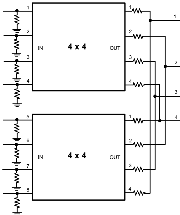
Figure 61. Input Expansion with Separate Termination Resistors
