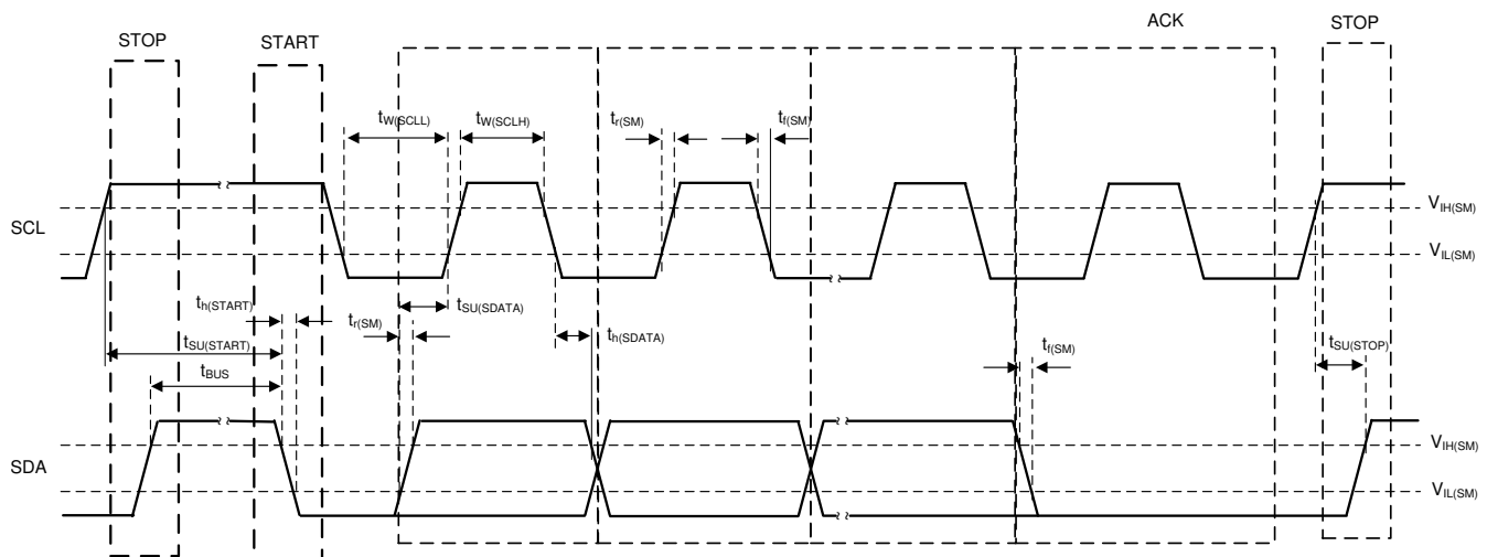
Figure 6-2. I²C Timing Diagram
