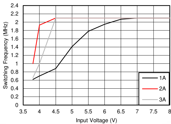
Figure 8-11. Typical Switching Frequency in Dropout Mode V_{OUT} = 3.3\text{ V} , f_{SW} = 2.1\text{ MHz}
