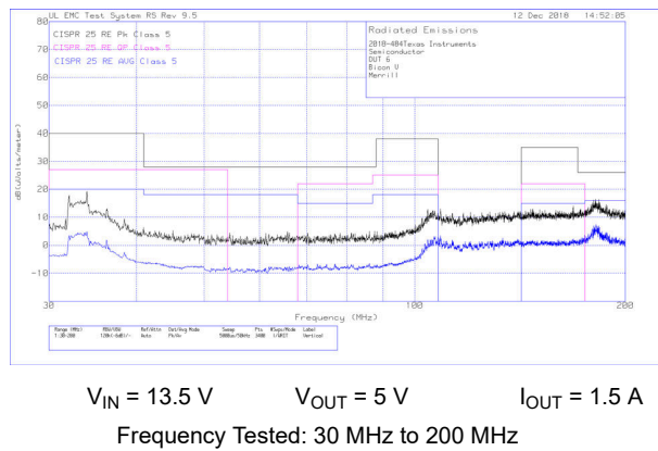
Figure 9-14. Radiated EMI Bicon Vertical vs. CISPR25 Limits
