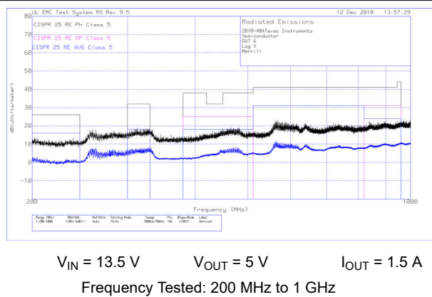
Figure 9-16. Radiated EMI Log Vertical vs. CISPR25 Limits
