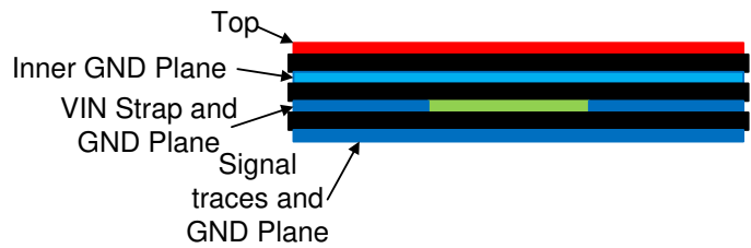
Figure 10-3. Example Layout for 400kHz, Adjustable Output
