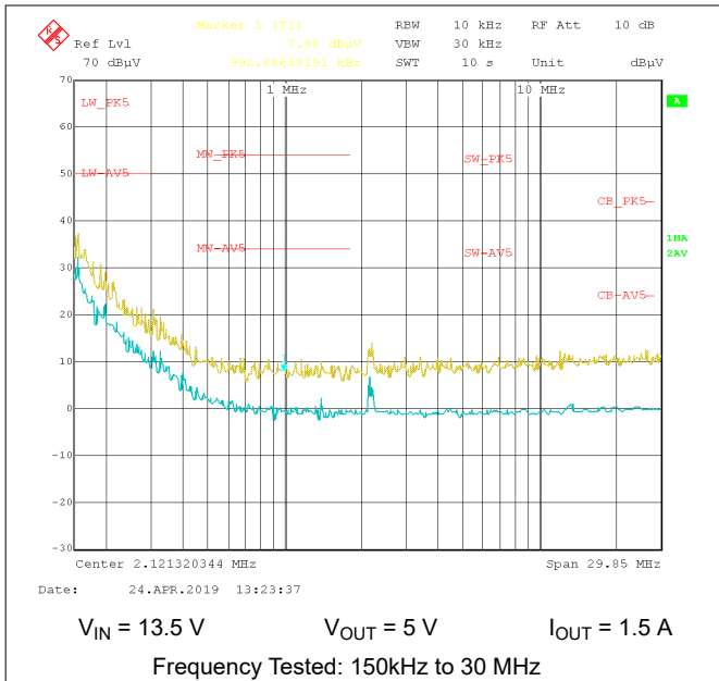
Figure 9-11. Conducted EMI vs. CISPR25 Limits (Yellow: Peak Signal, Blue: Average Signal)
