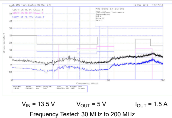
Figure 9-15. Radiated EMI Bicon Horizontal vs. CISPR25 Limits
