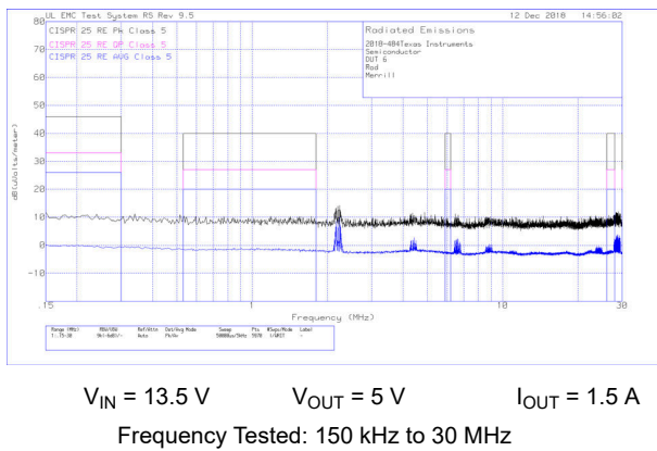
Figure 9-13. Radiated EMI Rod vs. CISPR25 Limits
