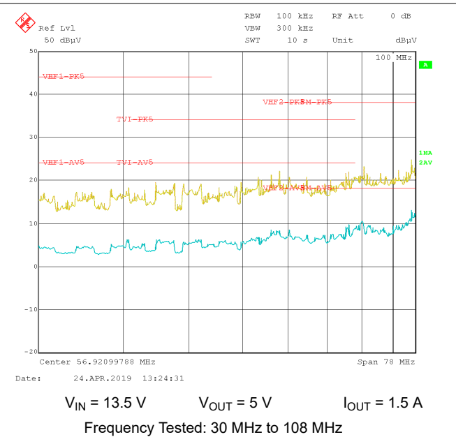
Figure 9-12. Conducted EMI vs. CISPR25 Limits (Yellow: Peak Signal, Blue: Average Signal)
