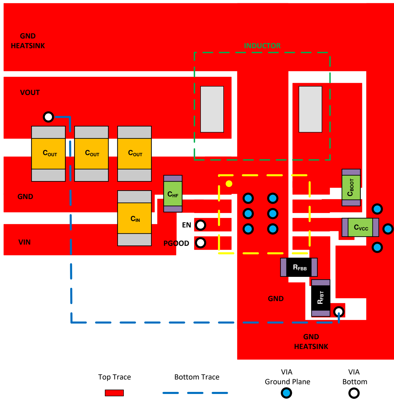
Figure 8-24. Example Layout
