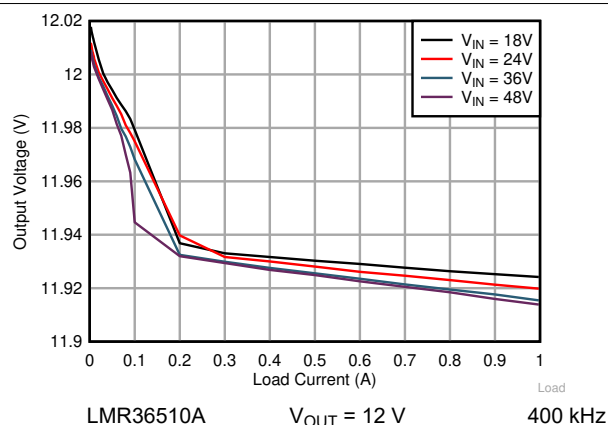
Figure 8-9. Load Regulation
