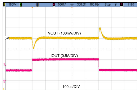
Figure 8-17. Load Transient
