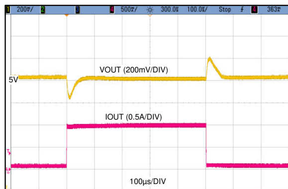
Figure 8-16. Load Transient
