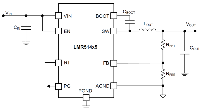
Simplified Schematic
