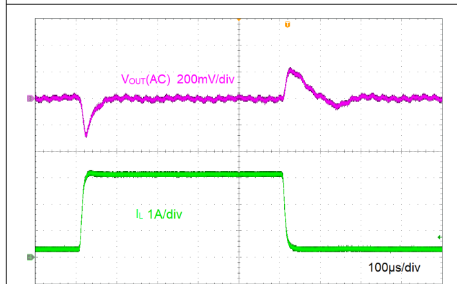
Figure 8-6. Load Transient
