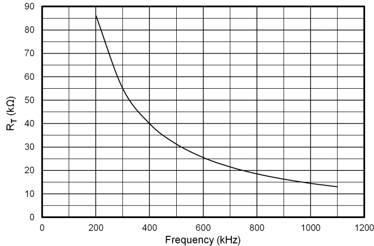
Figure 7-4. R_T Versus Frequency Curve
