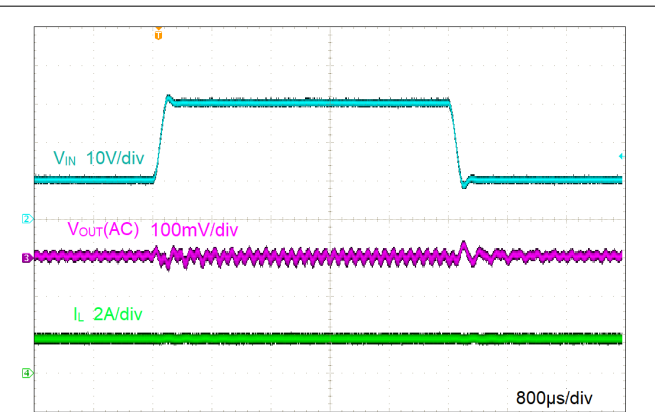
Figure 8-7. Line Transient
