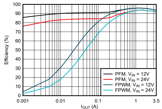
Efficiency vs Output Current V_{OUT} = 5V, 500kHz
