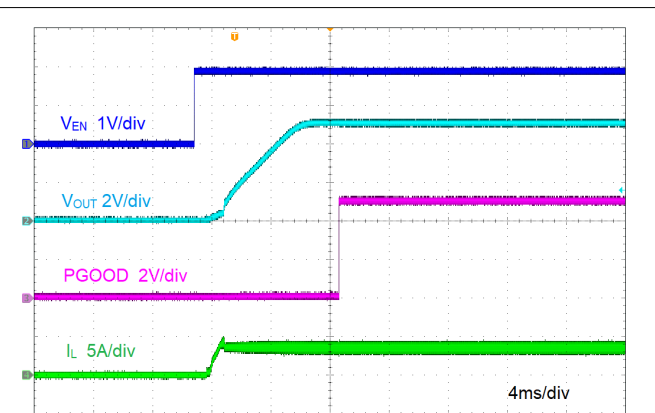
Figure 8-5. Start-Up by EN
