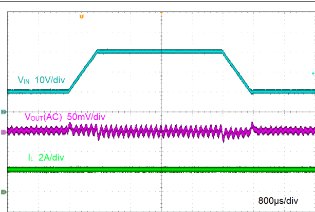
Figure 8-7. Line Transient
