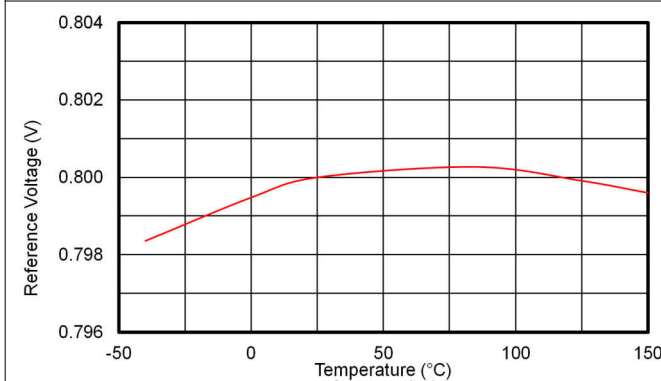
Figure 7-11. Reference Voltage
