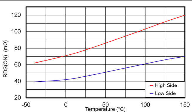
Figure 7-12. High Side and Low Side Switches R Ds_on
