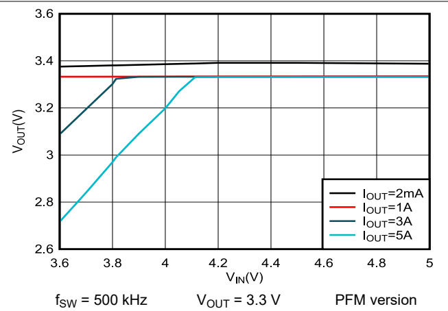
Figure 7-8. 3.3-V Dropout
