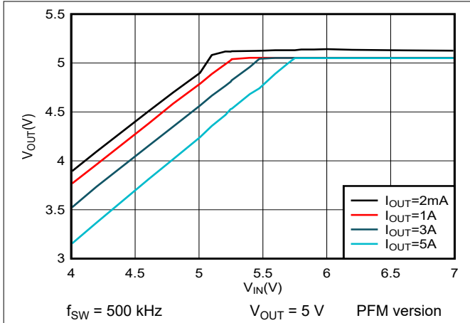
Figure 7-7. 5-V Dropout
