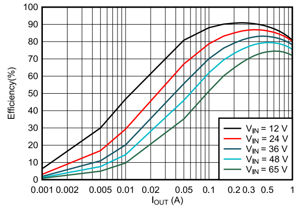
Figure 6-2. 3.3-V FPWM Efficiency Versus Load Current
