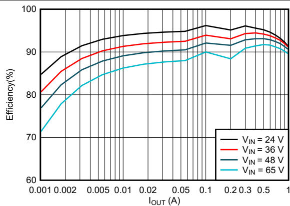
Figure 6-3. 5-V PFM Efficiency Versus Load Current
