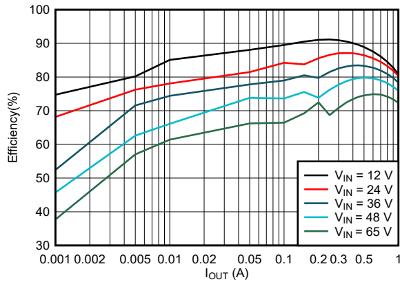
Figure 6-1. 3.3-V PFM Efficiency Versus Load Current
