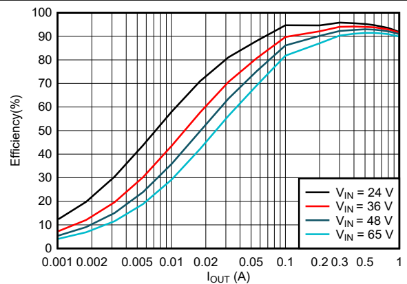
Figure 6-4. 5-V FPWM Efficiency Versus Load Current
