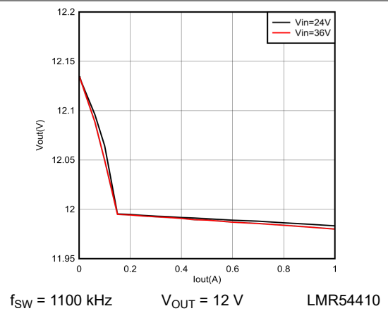
Figure 6-8. 12-V Load Regulation
