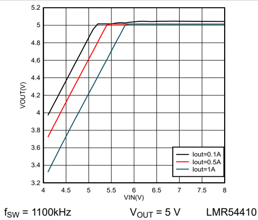
Figure 6-9. 5-V Dropout
