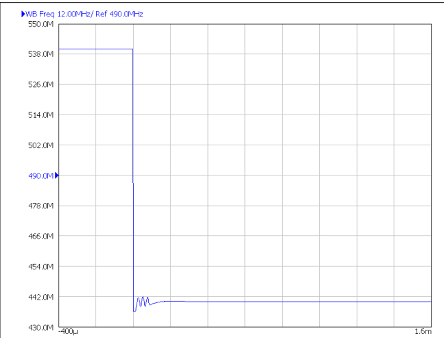
Figure 8-31. Internal VCO to External VCO Switching
