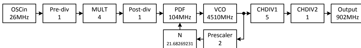
Figure 8-13. F1 Frequency Plan
