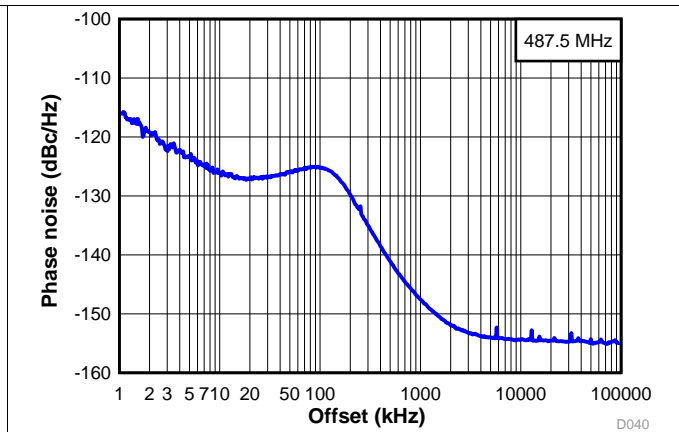
Figure 10. Wide Band Phase Noise at 487.5 MHz
