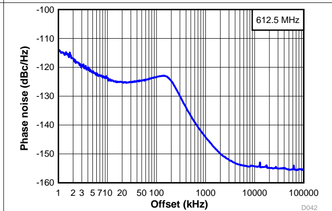
Figure 12. Wide Band Phase Noise at 612.5 MHz
