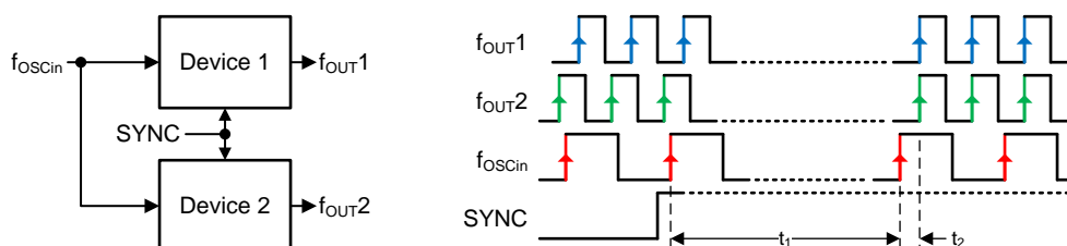
Figure 23. Phase Synchronization
