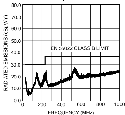
Figure 39. Radiated Emissions (EN 55022 Class B) from Evaluation Board
