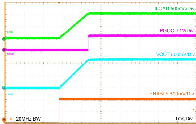
Figure 25. Startup V_{OUT} = 1.2\text{ V}
