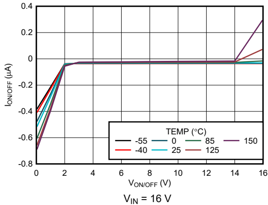
Figure 5-39. \text{ON}/\overline{\text{OFF}} Pin Current vs V_{\text{ON/OFF}} (New Chip)
