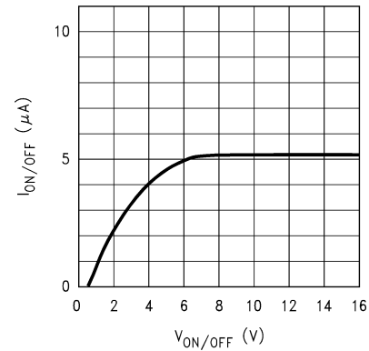
Figure 5-38. \text{ON}/\overline{\text{OFF}} Pin Current vs V_{\text{ON/OFF}} (Legacy Chip)
