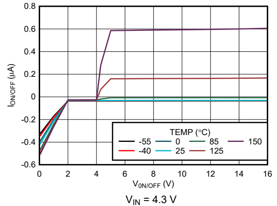
Figure 5-40. \text{ON}/\overline{\text{OFF}} Pin Current vs V_{\text{ON/OFF}} (New Chip)
