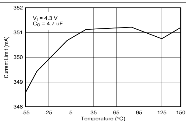
Figure 5-18. Instantaneous Short Circuit Current vs Temperature (New Chip)
