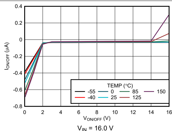
Figure 5-28. ON/ OFF Pin Current vs V_{ON/ OFF} (New Chip)
