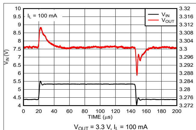
Figure 7-7. Line Transient Response (New Chip)
