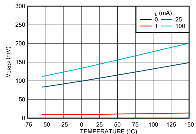
Dropout Voltage vs Temperature (New Chip)
