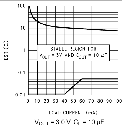
Figure 7-6. 3.0-V, 10- \mu\text{F} ESR Curves (Legacy Chip)
