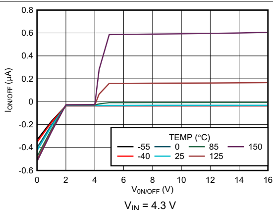
Figure 5-27. ON/ OFF Pin Current vs V_{ON/ OFF} (New Chip)
