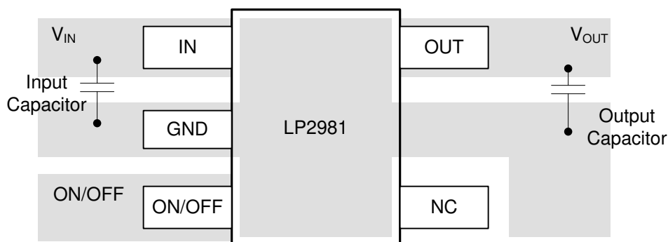
Figure 9-1. Recommended Layout
