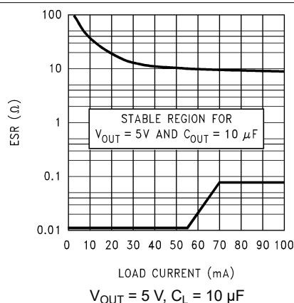
Figure 7-4. 5-V, 10- \mu\text{F} ESR Curves (Legacy Chip)
