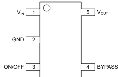
Figure 5-1. DBV Package, 5-Pin SOT-23 (Top View)
