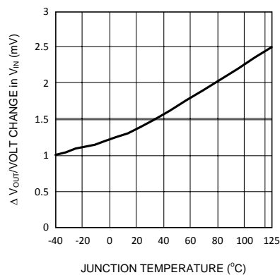
Figure 6. DC Line Regulation vs Temperature
