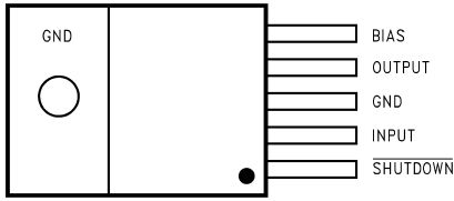
Figure 1. TO-220, Top View
