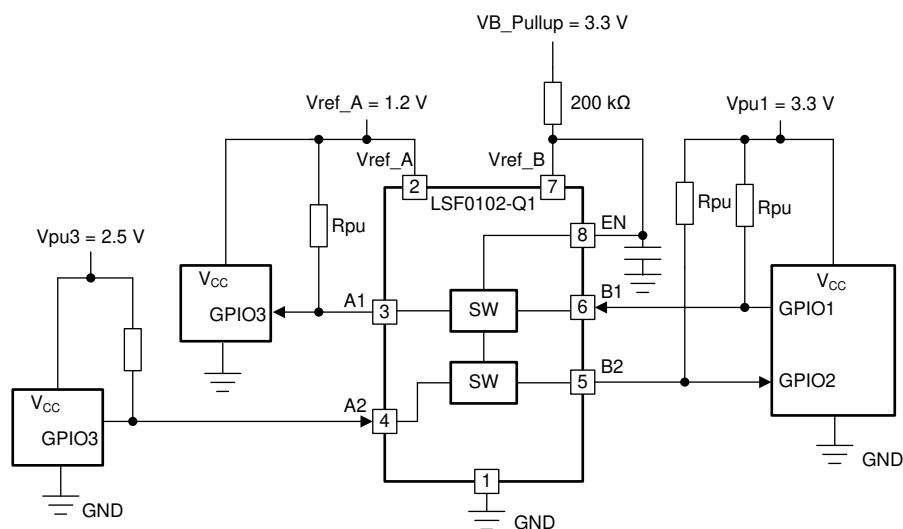
Figure 8-1. Bidirectional Translation to Multiple Voltage Levels
