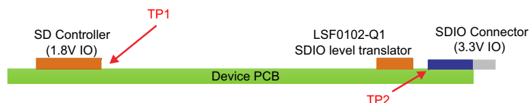
Figure 10-2. Device Placement
