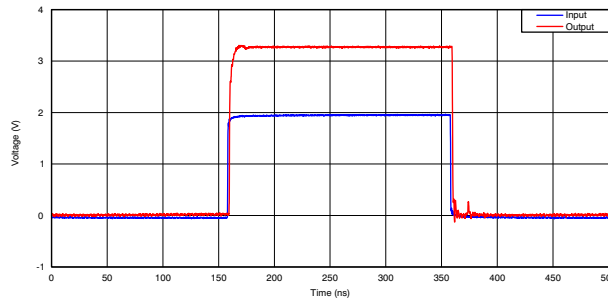
Figure 8-2. Captured Waveform From Above I 2 C Set-Up (1.8 V to 3.3 V at 2.5 MHz)
