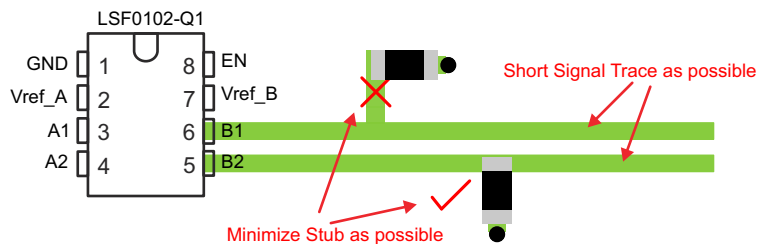
Figure 10-1. Short Trace Layout
