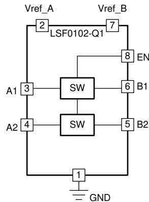
Figure 7-1. LSF0102-Q1 Functional Block Diagram
