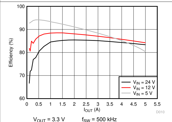
Figure 5-4. Efficiency versus Load Current
