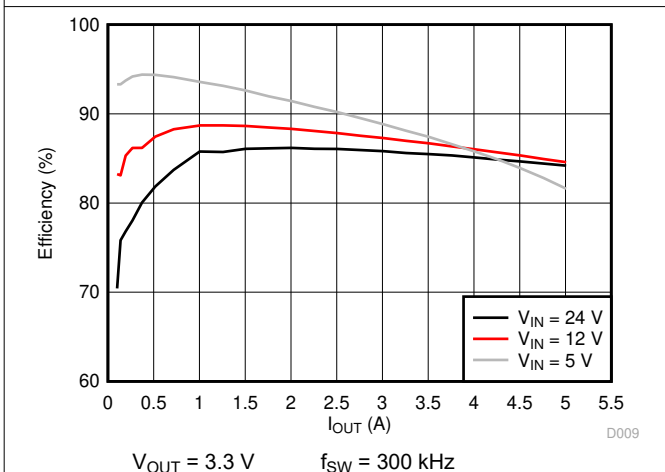
Figure 5-3. Efficiency versus Load Current
