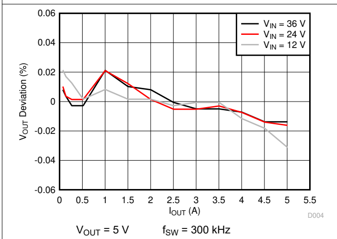
Figure 5-5. Load Regulation
