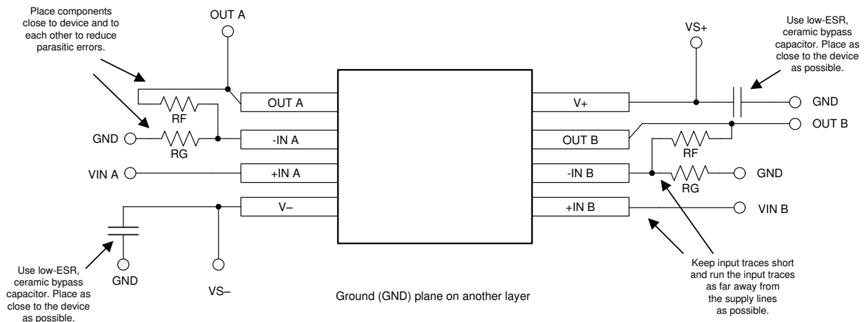
Figure 37. Layout Example
