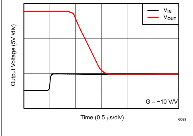
Figure 5-39. Positive Overload Recovery
