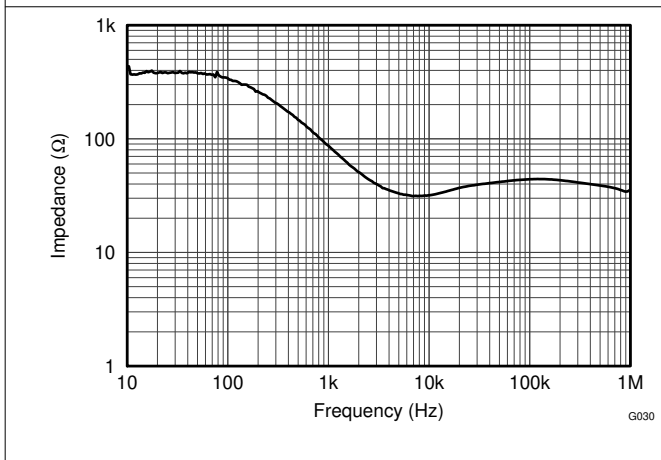
Figure 5-41. Open-Loop Output Impedance vs Frequency
