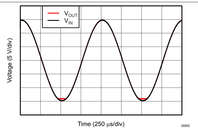
Figure 5-42. No Phase Reversal
