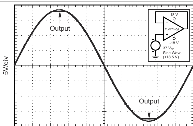
Time (100ms/div) Figure 6-25. No Phase Reversal
