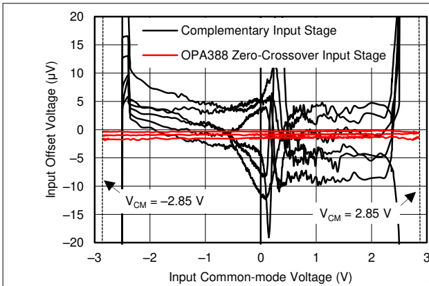
Figure 7-1. Input Crossover Distortion Nonlinearity
