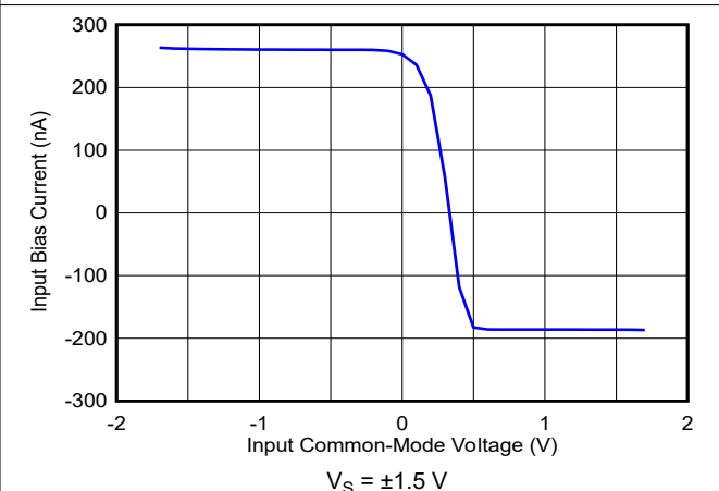
Figure 6-33. Input Bias Current vs Input Common-Mode Voltage
