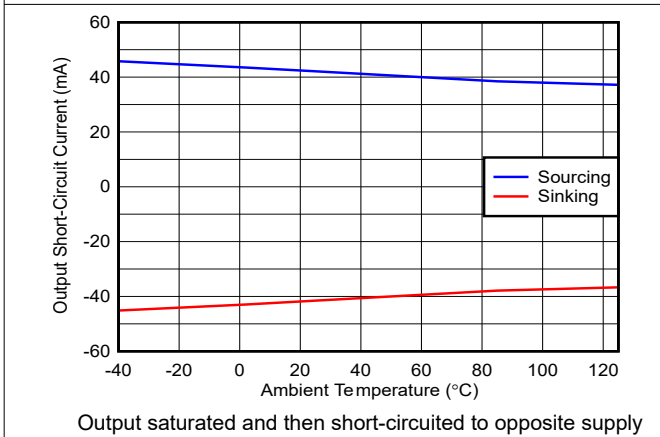
Figure 6-15. Output Short-Circuit Current vs Ambient Temperature
