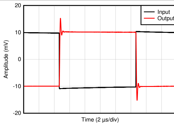
Figure 5-36. Negative Overload Recovery
