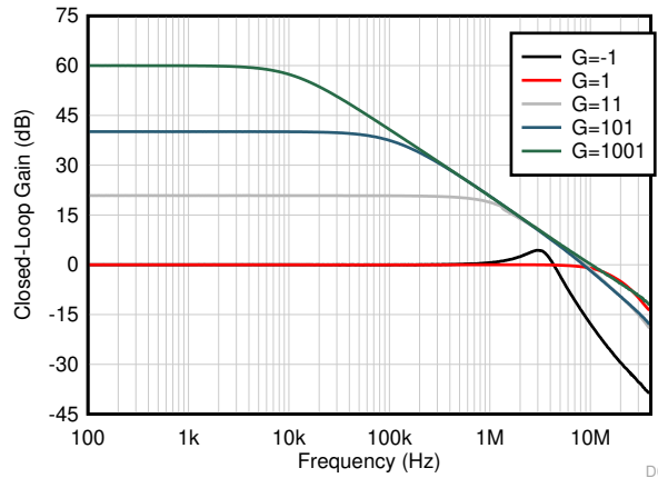
Figure 5-12. Closed-Loop Gain vs Frequency
