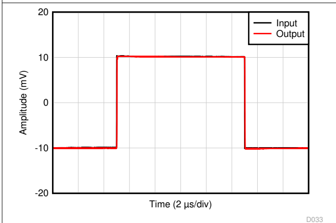
Figure 5-35. Positive Overload Recovery
