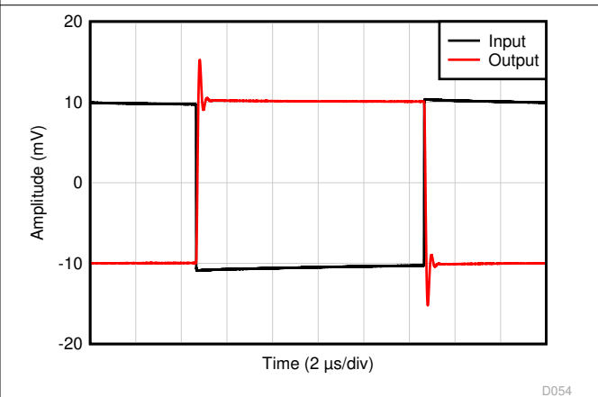
Figure 5-36. Negative Overload Recovery
