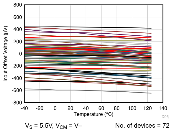
Figure 6-7. Input Offset Voltage vs Temperature
