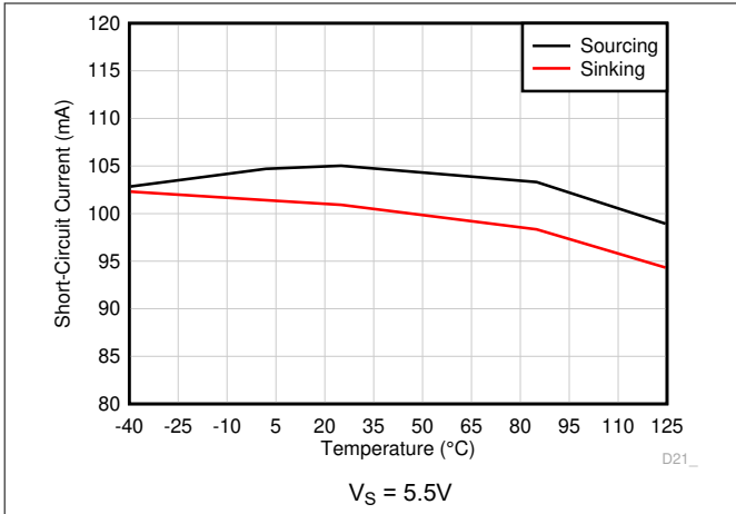
Figure 6-67. Short-Circuit Current vs Temperature
