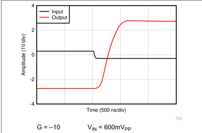
Figure 6-57. Overload Recovery
