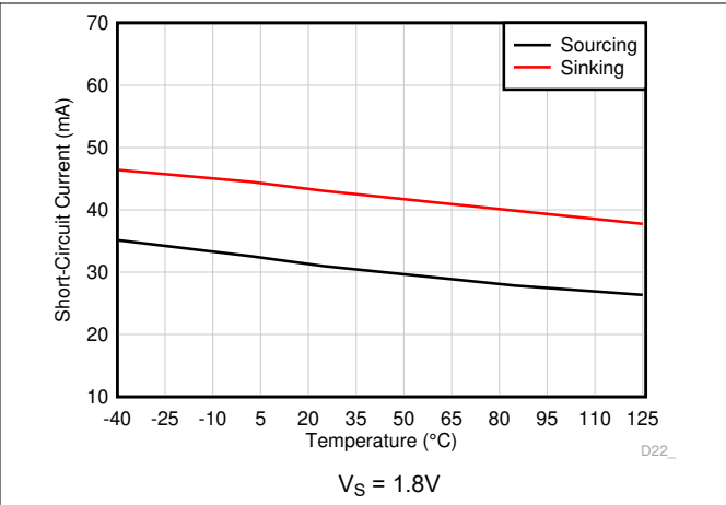
Figure 6-68. Short-Circuit Current vs Temperature
