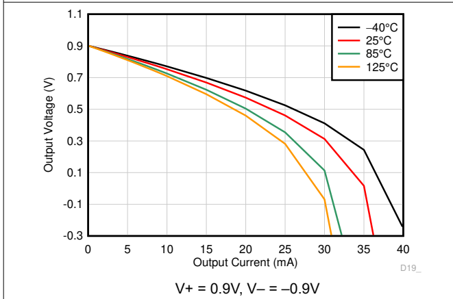
Figure 6-27. Output Voltage Swing vs Output Current (Sourcing)
