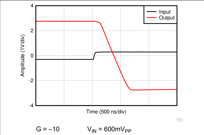
Figure 6-58. Overload Recovery
