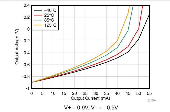
Figure 6-28. Output Voltage Swing vs Output Current (Sinking)
