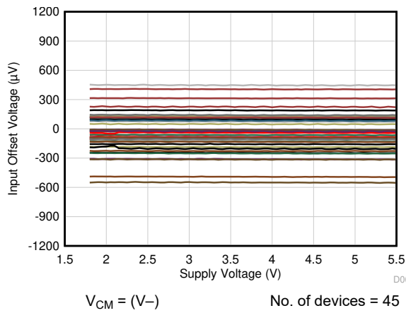
Figure 6-7. Input Offset Voltage vs Supply Voltage
