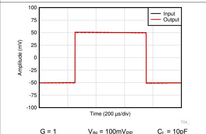
Figure 6-60. Small-Signal Step Response
