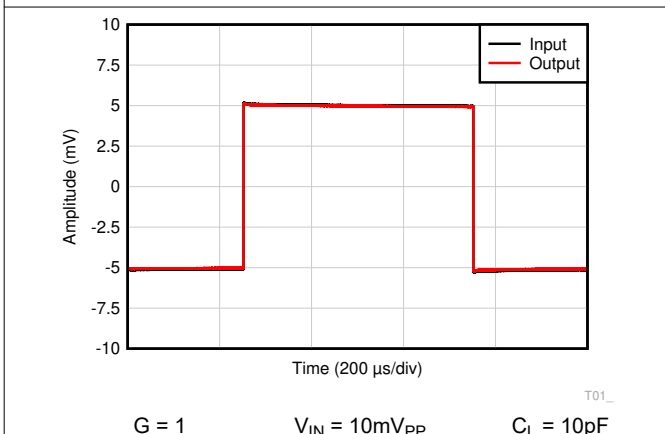
Figure 6-59. Small-Signal Step Response
