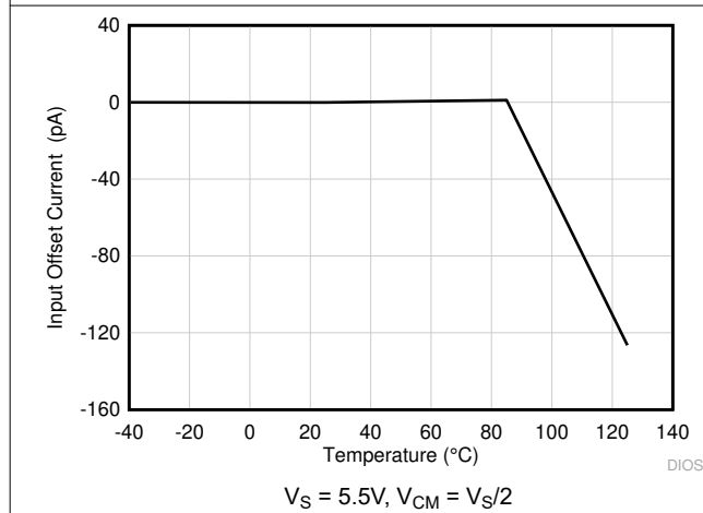
Figure 6-15. I_{OS} vs Temperature
