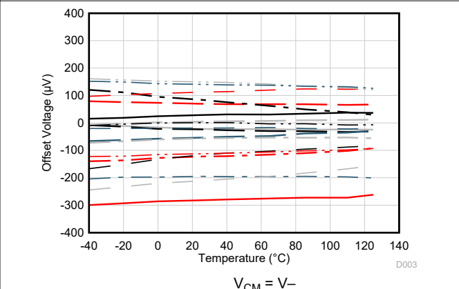
Figure 6-4. Offset Voltage vs Temperature
