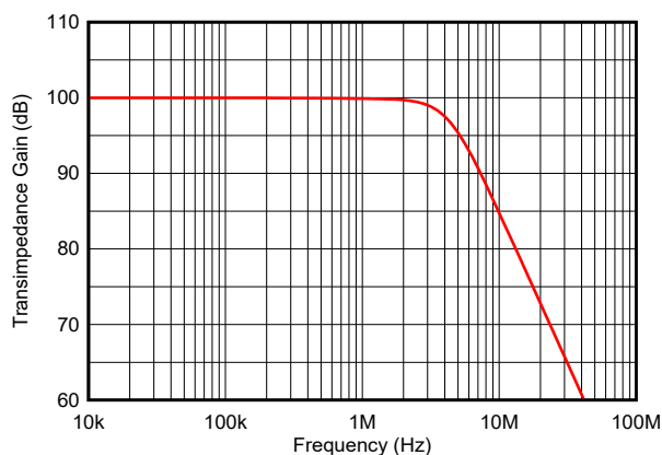
100-kΩ Transimpedance Bandwidth
