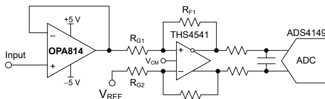
High-Input-Impedance Digitizer Front End
