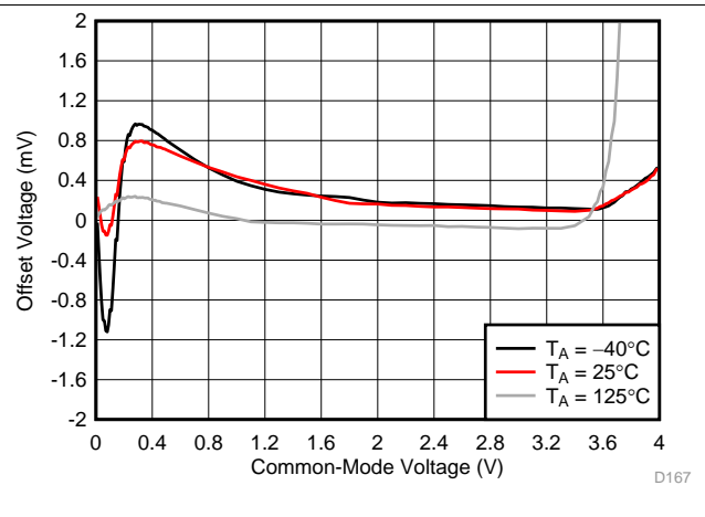
Figure 34. Offset Voltage vs Input Common-Mode Voltage vs Ambient Temperature
