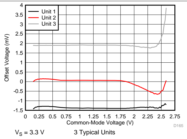
Figure 32. Offset Voltage vs Input Common-Mode Voltage
