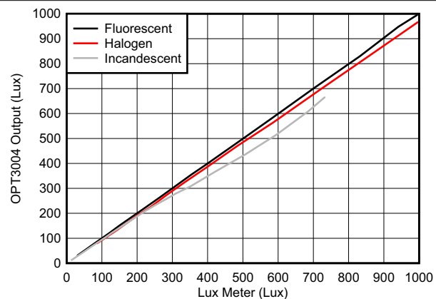
Figure 9-6. Compensated Output of the OPT3004 Under a Dark Window Illuminated by Fluorescent, Halogen, and Incandescent Light Sources
