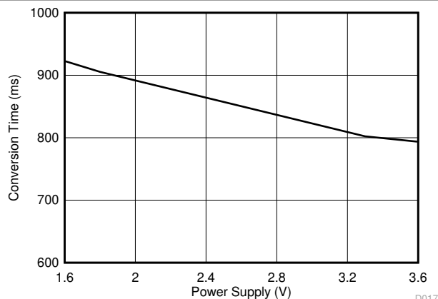
Figure 7-5. Conversion Time vs Power Supply
