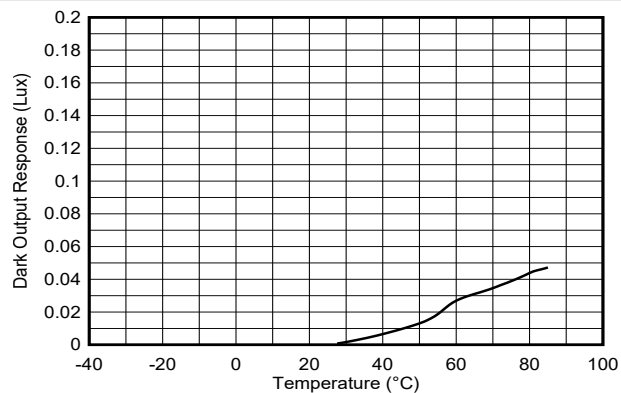
Figure 7-3. Dark Response vs Temperature
