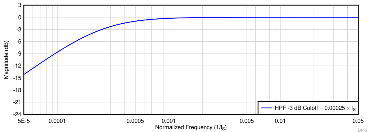
Figure 6-10. HPF Filter Frequency Response Plot
