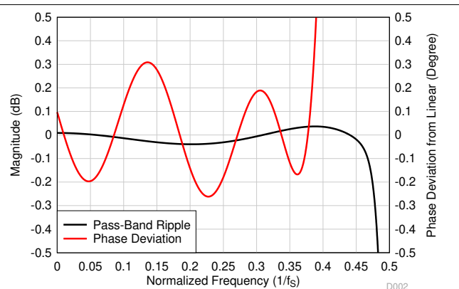
Figure 6-30. Low-Latency Decimation Filter Pass-Band Ripple and Phase Deviation
