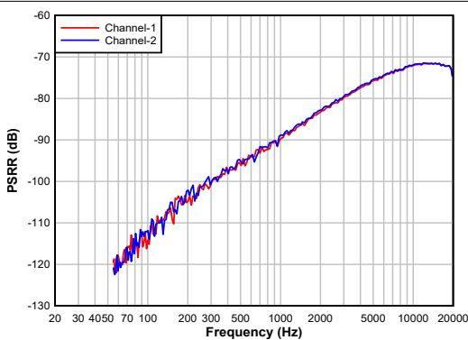
Figure 5-5. Single-ended Input: PSRR vs. Frequency with DC Coupled input
