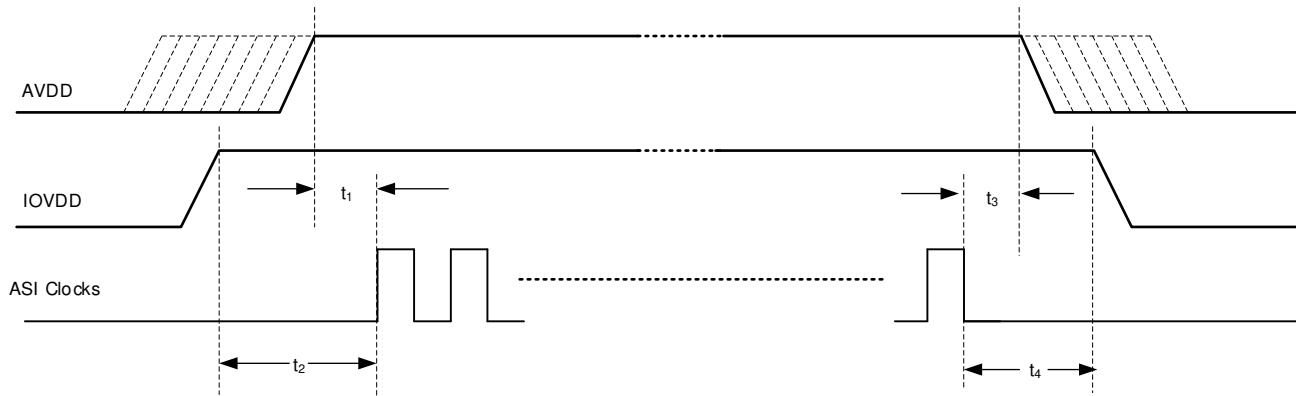
Figure 8-1. Power-Supply Sequencing Requirement Timing Diagram
