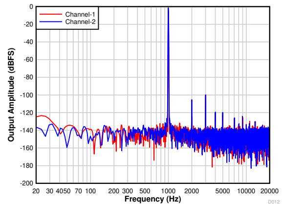
Figure 7-12. PCM1820-Q1: FFT With a -1-dBr Input
