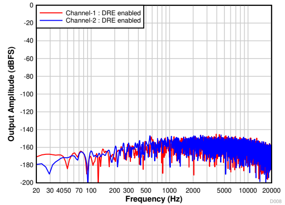
Figure 7-8. PCM1820-Q1: FFT With Idle Input and DRE Enabled
